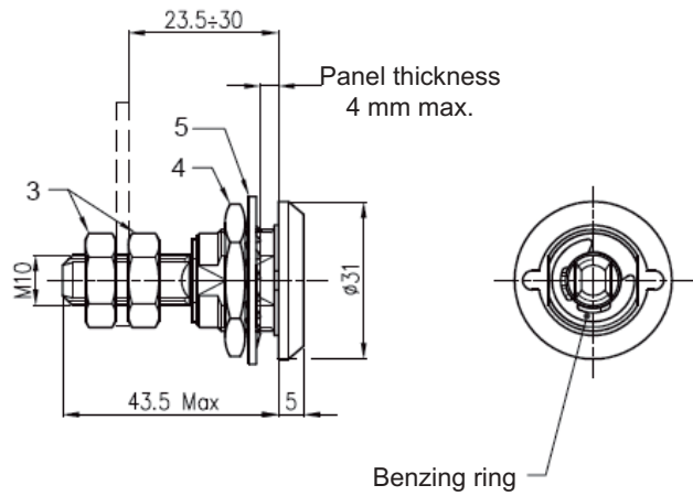
Slotted recess
